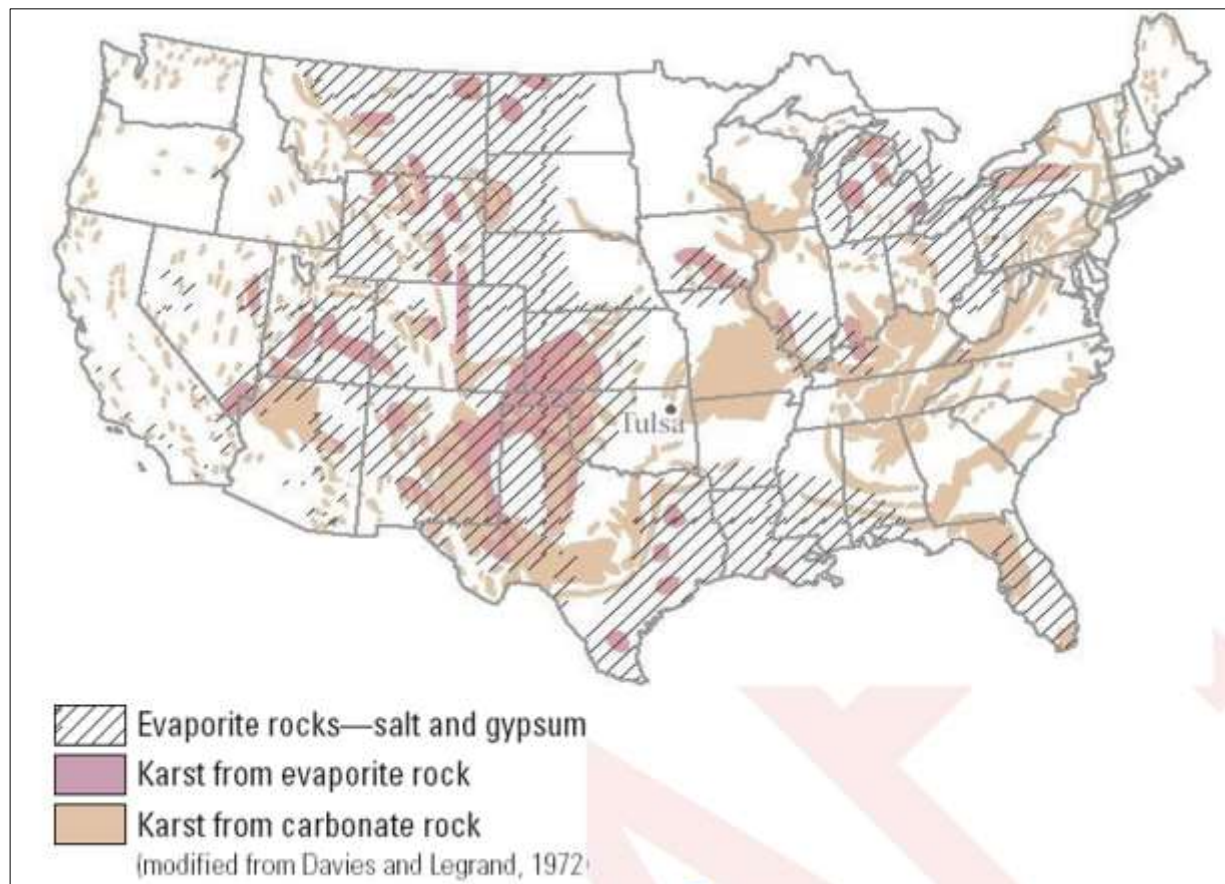
Figure 43. Land Subsidence in the United States
