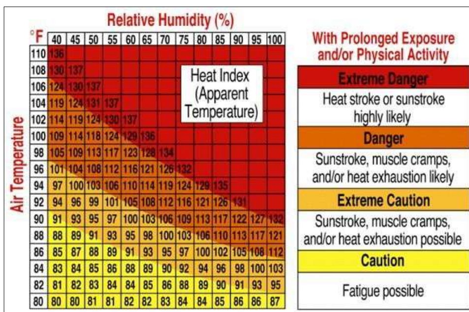
Figure 25. Heat Index Chart ( NWS )
