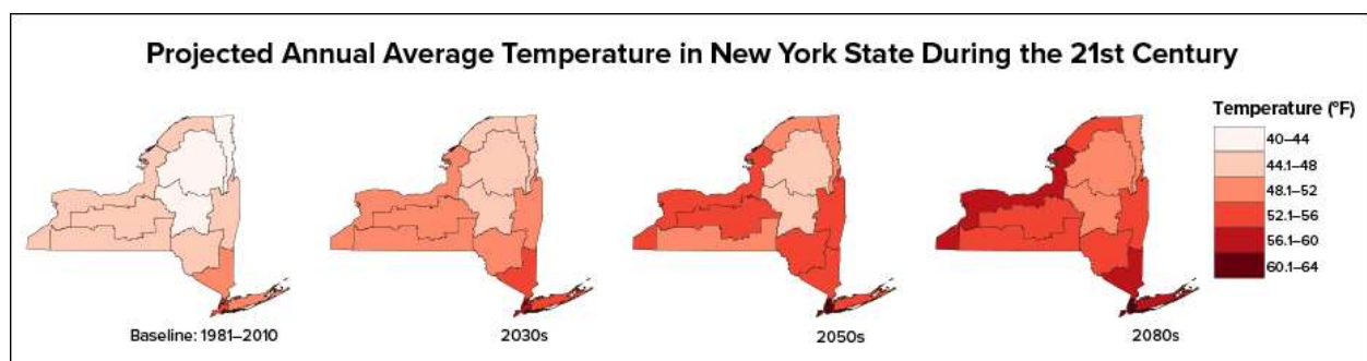
Figure 26. Projected Changes to Annual Average Temperatures New York
