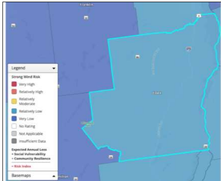
Figure 21. High Wind National Risk Score
