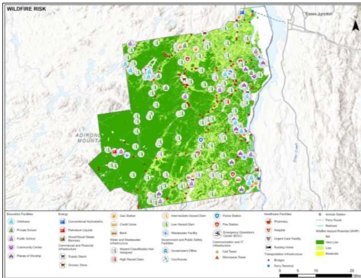
Figure 28. Wildfire Risk Map
